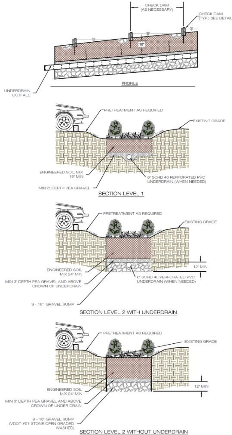
Figure GIP-05-03. Typical Details for Level 1 and 2 Water Quality Swales (source: VADCR, 2011)
