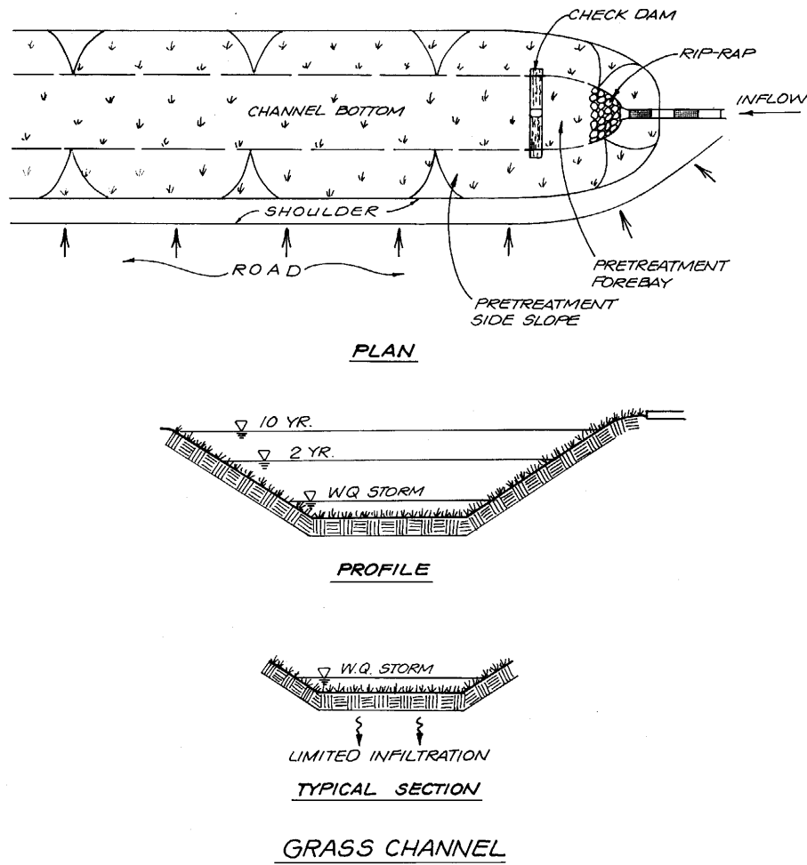
Figure TSS-07-01 Typical Grass Channel
