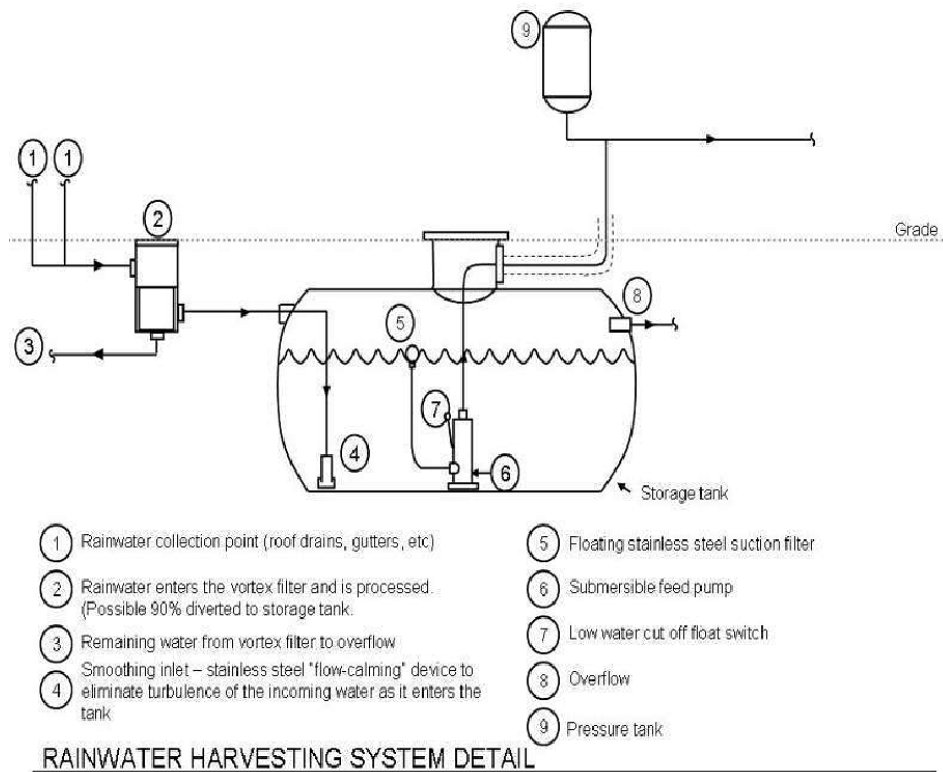
Figure GIP-11-07. Sample Rainwater Harvesting System Detail (Source: VADCR, 2011)
