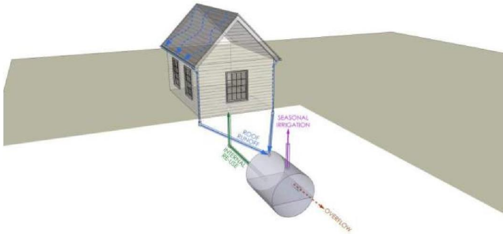
Figure GIP-11-01. Configuration 1: Year-round indoor use with optional seasonal outdoor use (Source: VADCR, 2011)
