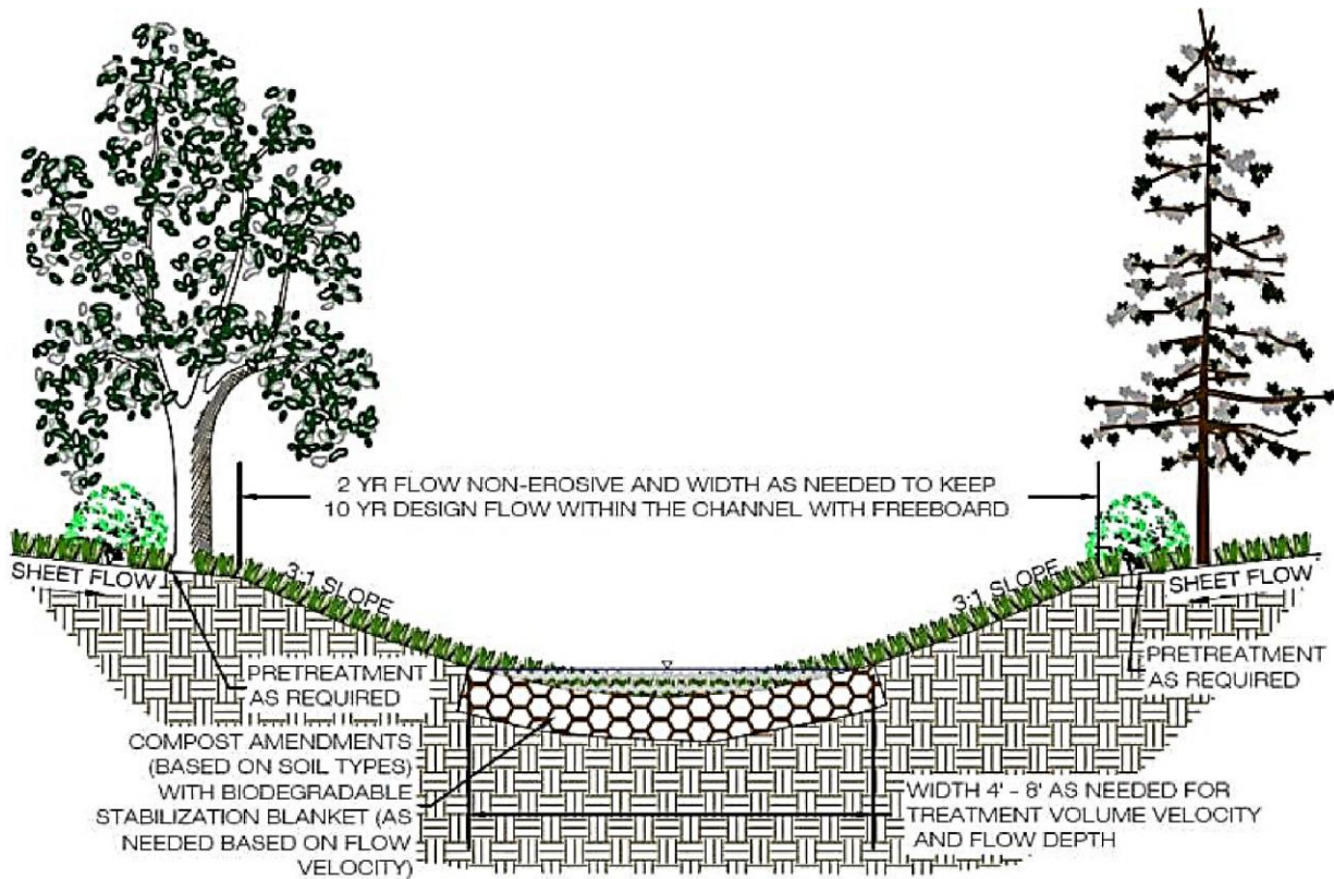
Figure GIP-08-04: Grass Channel with Compost Amendments - Section
