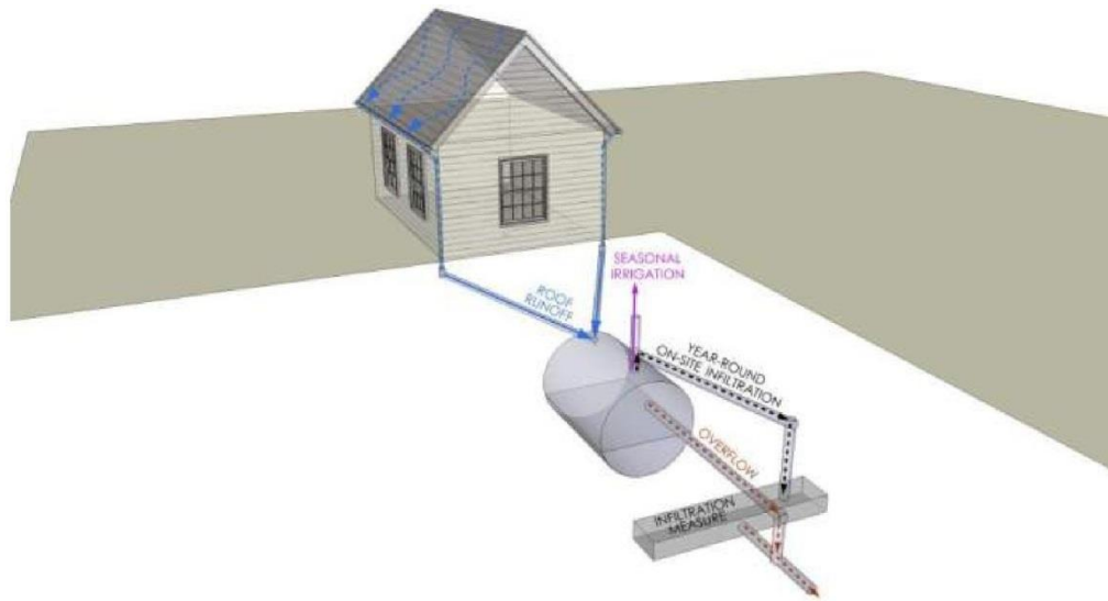
Figure GIP-11-02. Configuration 2: Seasonal outdoor use and approved year-round secondary practice (Source: VADCR, 2011)
