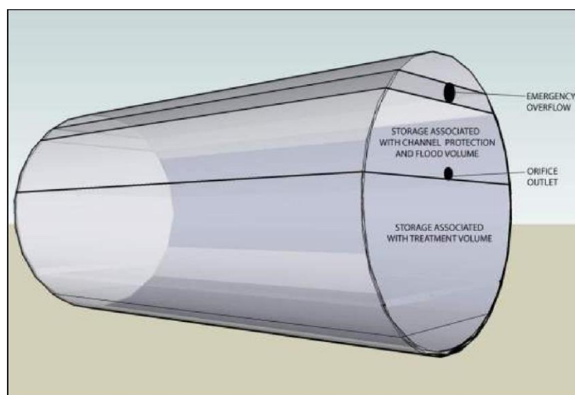
Figure GIP-11-05. Tank Design 2: Storage Associated with Treatment, Channel Protection and Flood Volume (Source: VADCR, 2011)
