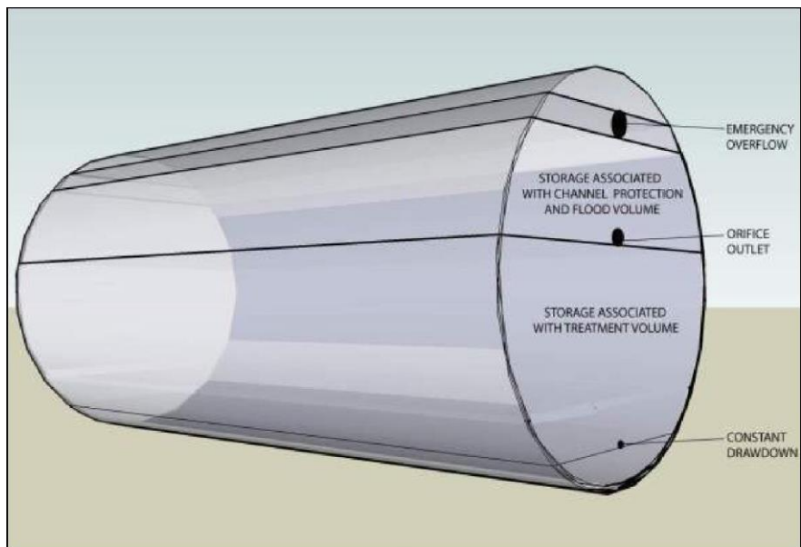
Figure GIP-11-06. Tank Design 3: Constant drawdown, Storage Associated with Treatment, Channel Protection and Flood Volume (Source: VADCR, 2011)
