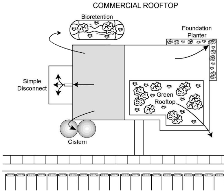
Figure GIP-07-01. Roof Disconnection with Alternative Runoff Reduction Practices (Source: VADCR, 2011)
