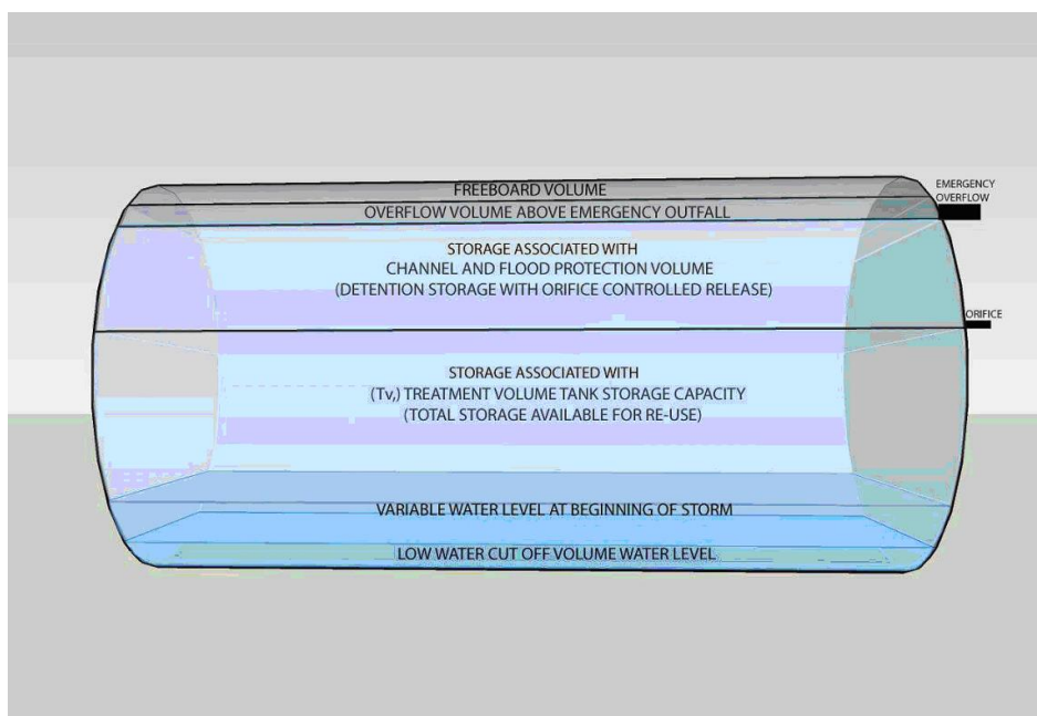
Figure GIP-11-15. Incremental Design Volumes associated with tank sizing (Source: VADCR, 2011)
