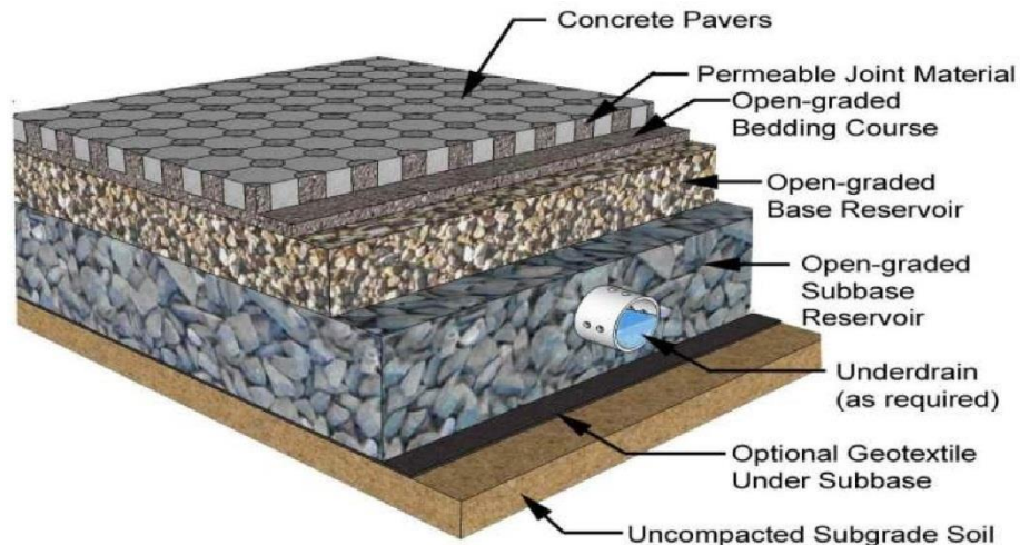
Figure GIP-03-02. Typical Detail of Concrete Paver (Source: Smith, 2009)
