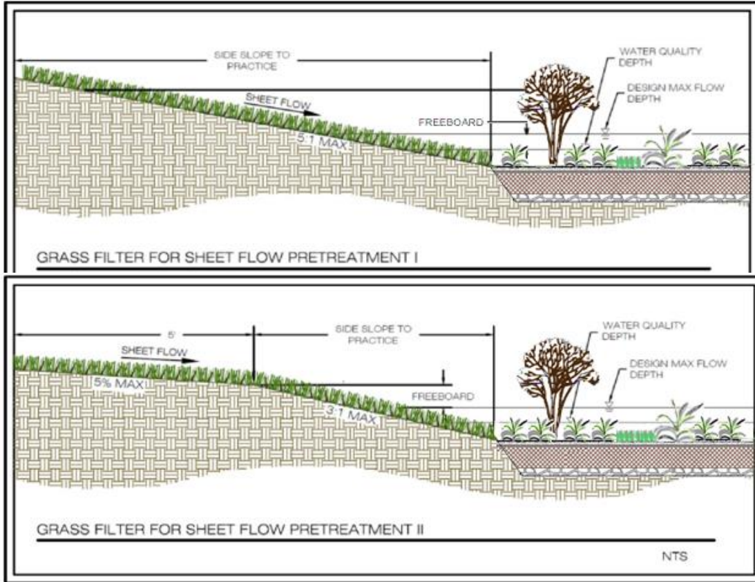
Figure GIP-01-04. Pretreatment Option - Grass Filter for Sheet Flow (source: VADCR, 2010)
