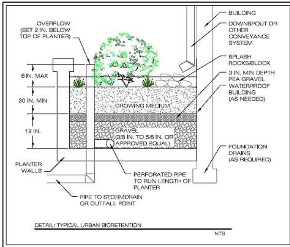
Figure GIP-02-04. Stormwater Planter Cross-Section (source: VADCR, 2010)
