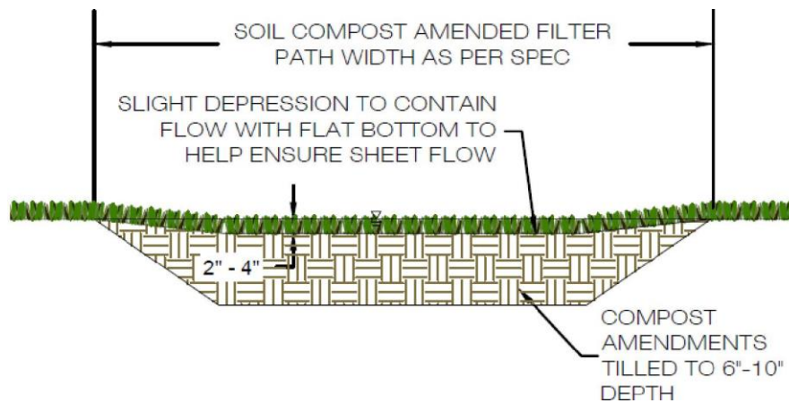
Figure GIP-07-02. Disconnection: Soil Compost Amended Filter Path (Source: VADCR, 2011)
