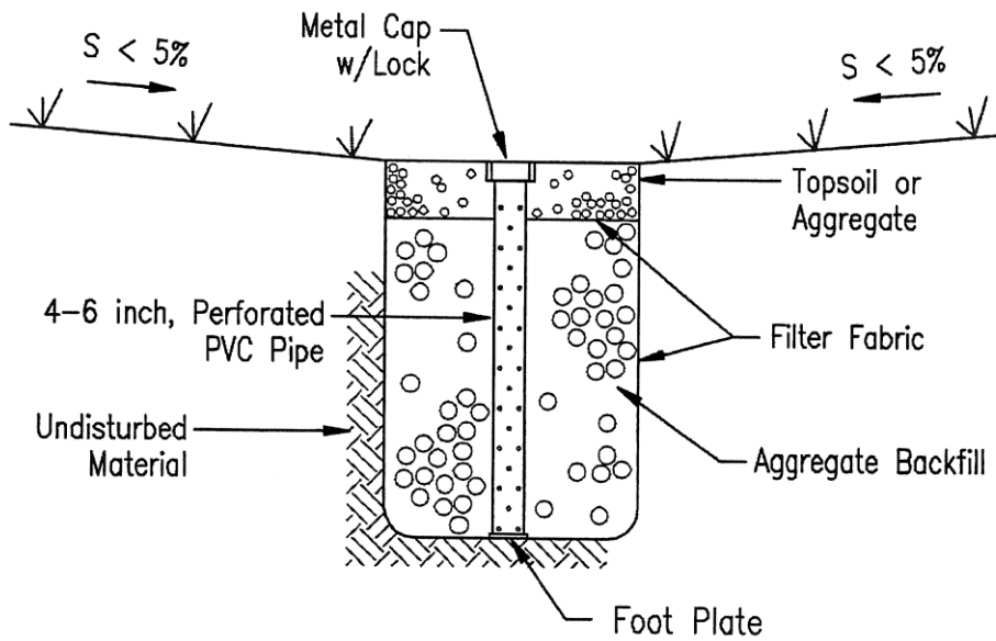
Figure GIP-04-04. Observation Well Detail (VADCR, 2011)
