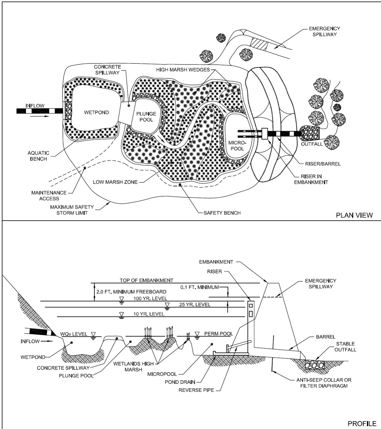
Figure TSS-02-04. Schematic of Pond/Wetland System
