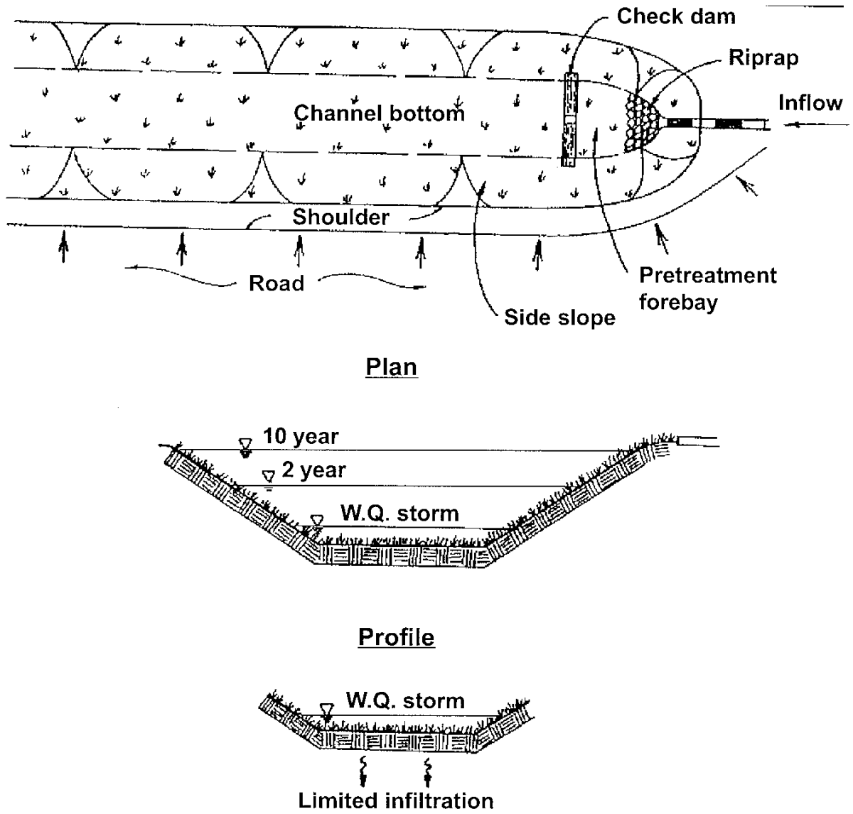
Figure GIP-08-01. Grass Channel – Typical Plan, Profile and Section
