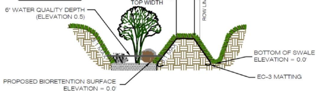
Figure GIP-01-11. Typical Details for Off-Line Bioretention (source: VADCR, 2010)
