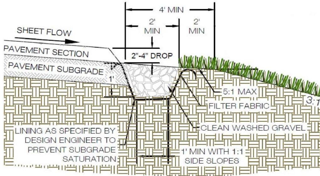
Figure GIP-09-06. Gravel Diaphragm – Sheet Flow Pre-treatment (source: VADCR, 2011)
