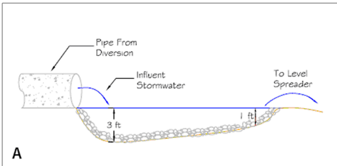
Figure GIP-09-02. Level Spreader Forebay (Hathaway and Hunt 2006)
