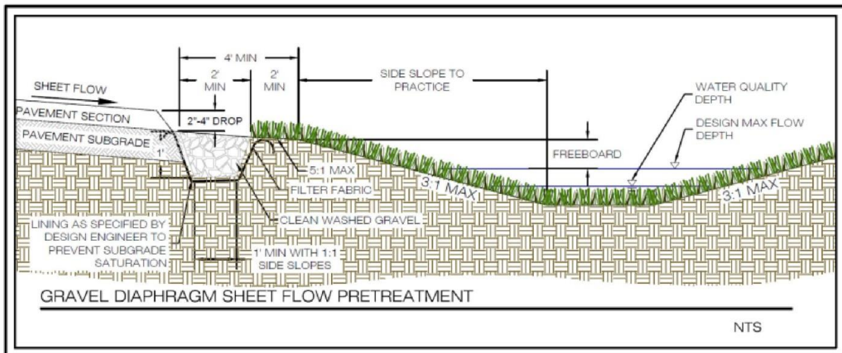
Figure GIP-05-06. Pretreatment – Gravel Diaphragm for Sheet Flow from Impervious or Pervious (source: VADCR, 2011)
