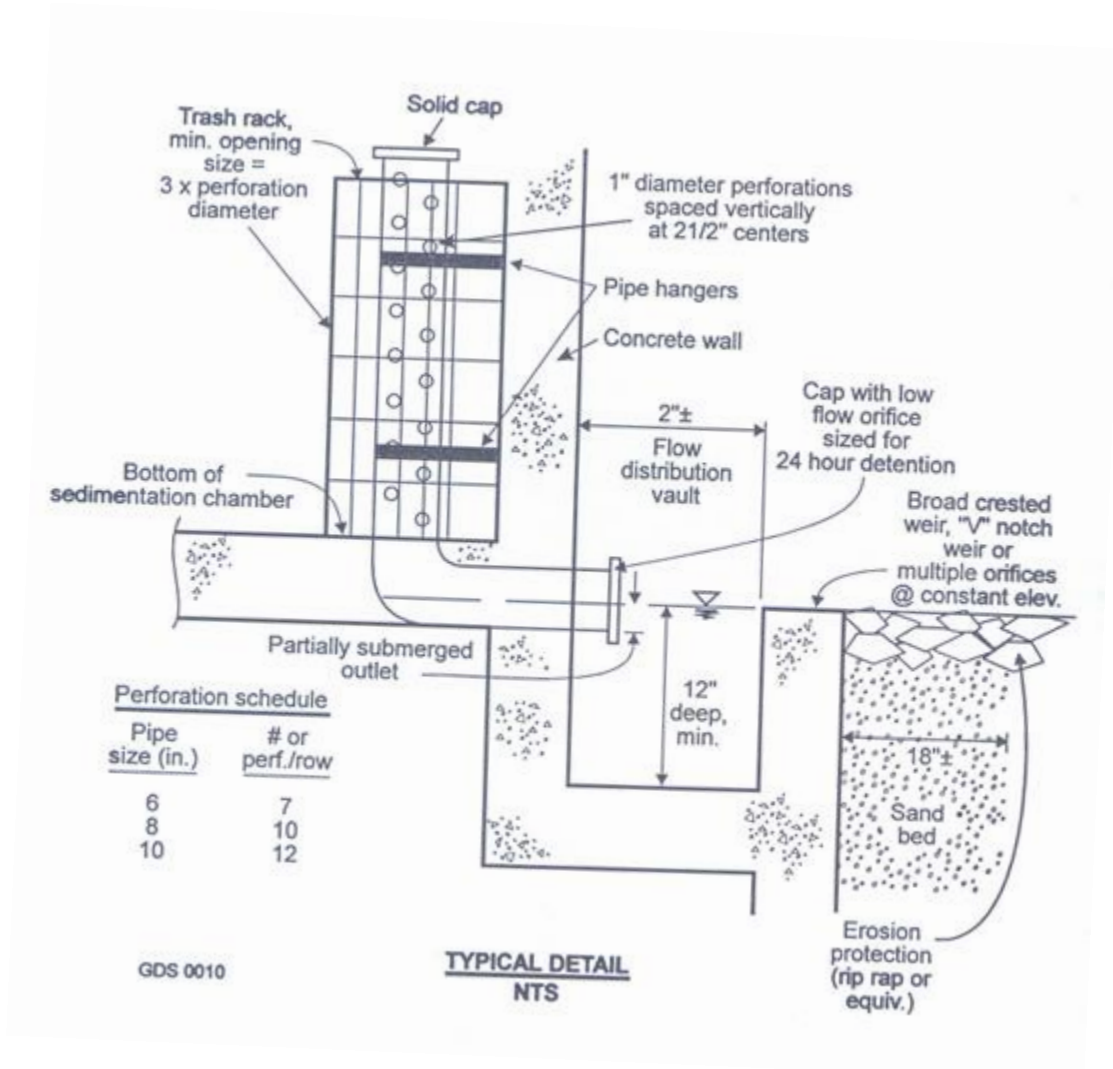
Figure TSS-03-04 Surface Sand Filter Perforated Stand-Pipe
