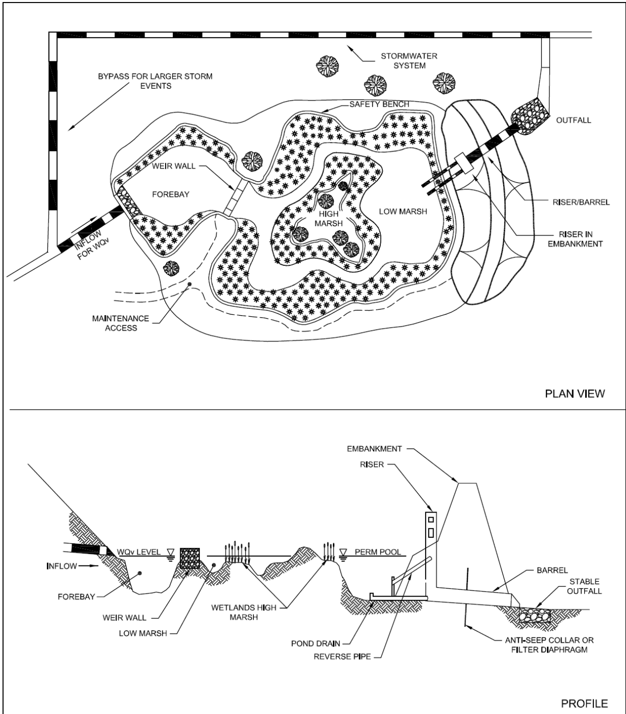
Figure TSS-02-07. Example of Off-line Constructed Wetland
