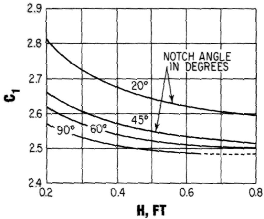
Figure TSS-01-08. Sharp-Crested V-Notch Weir Discharge Coefficients
