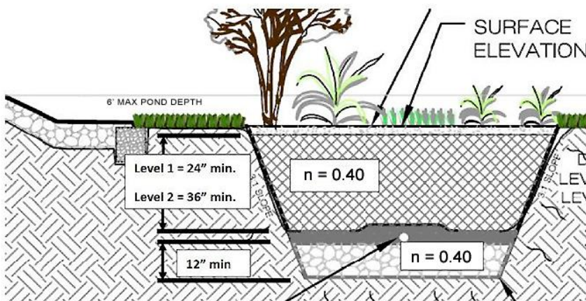
Figure GIP-01-07. Typical Level 2 Bioretention Section with Porosities for Volume Computations
