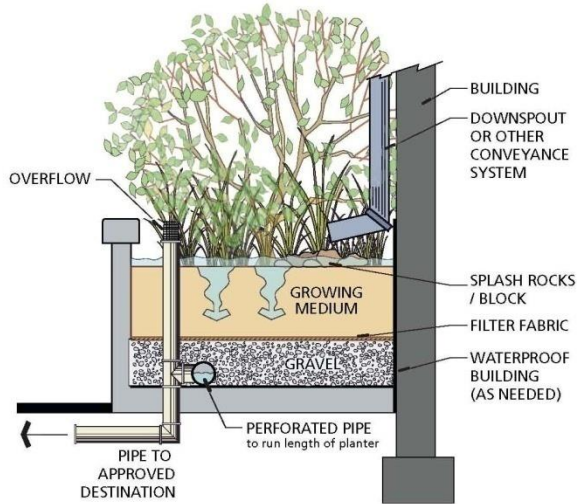
Figure GIP-02-06 Flow-through planter. (Source: Portland Bureau of Environmental Services)
