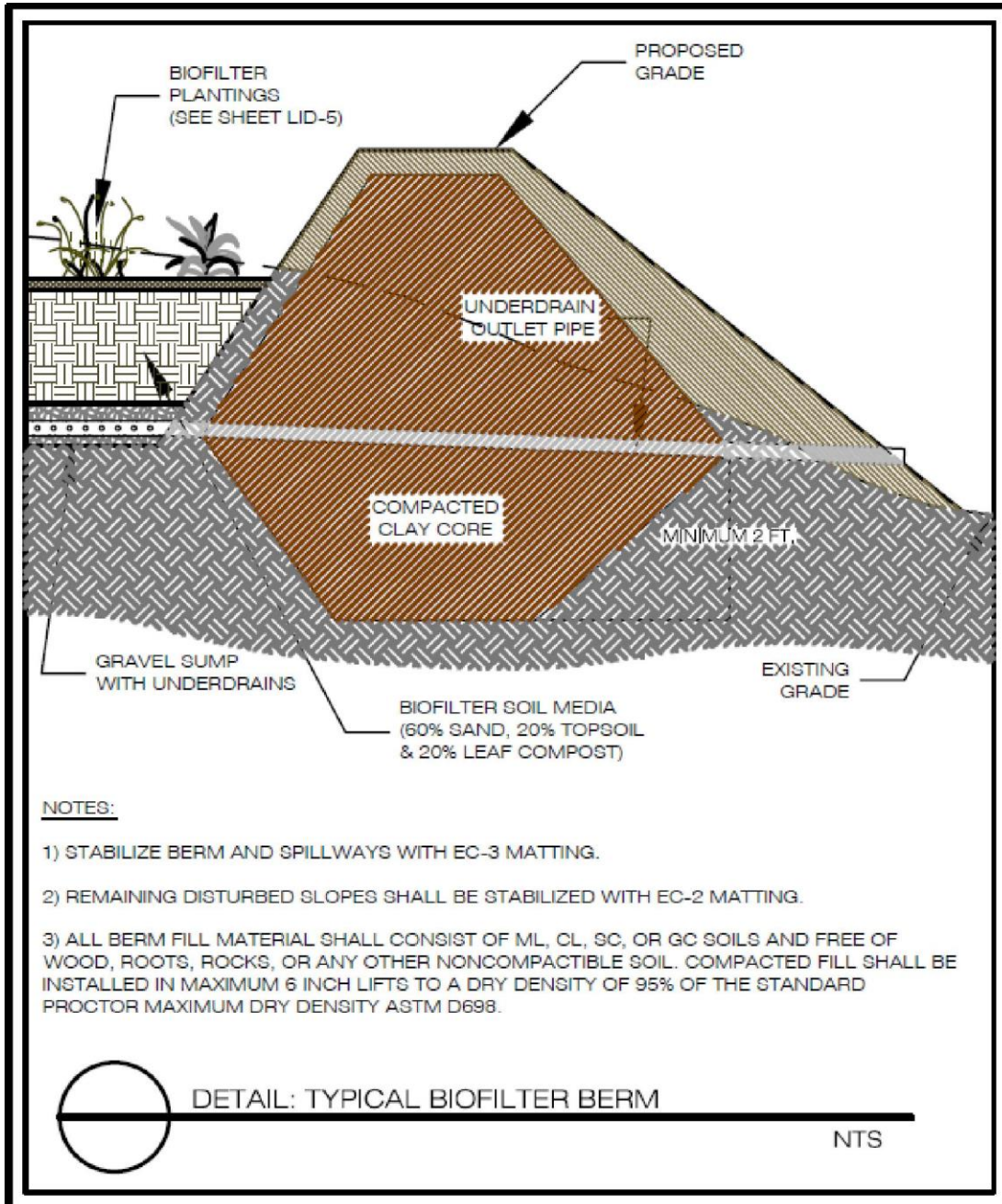
Figure GIP-01-B2. Typical Bioretention Basin Berm (source: VADCR, 2010)
