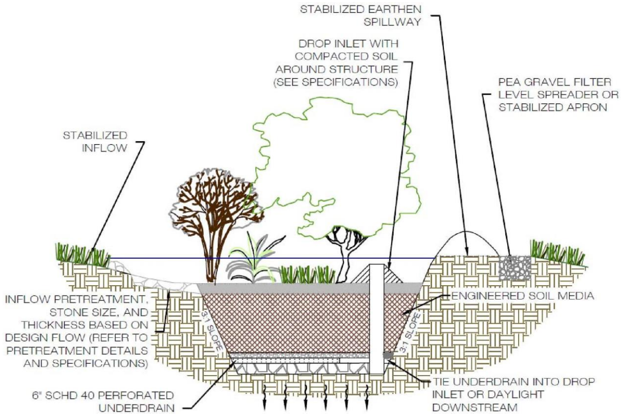
Figure GIP-01-B3. Typical Bioretention Basin – Inflow & Outflow – Section (source: VADCR, 2010)
