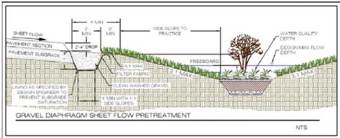
Figure GIP-01-05. Pretreatment Option – Gravel Diaphragm for Sheet (source: VADCR, 2010)
