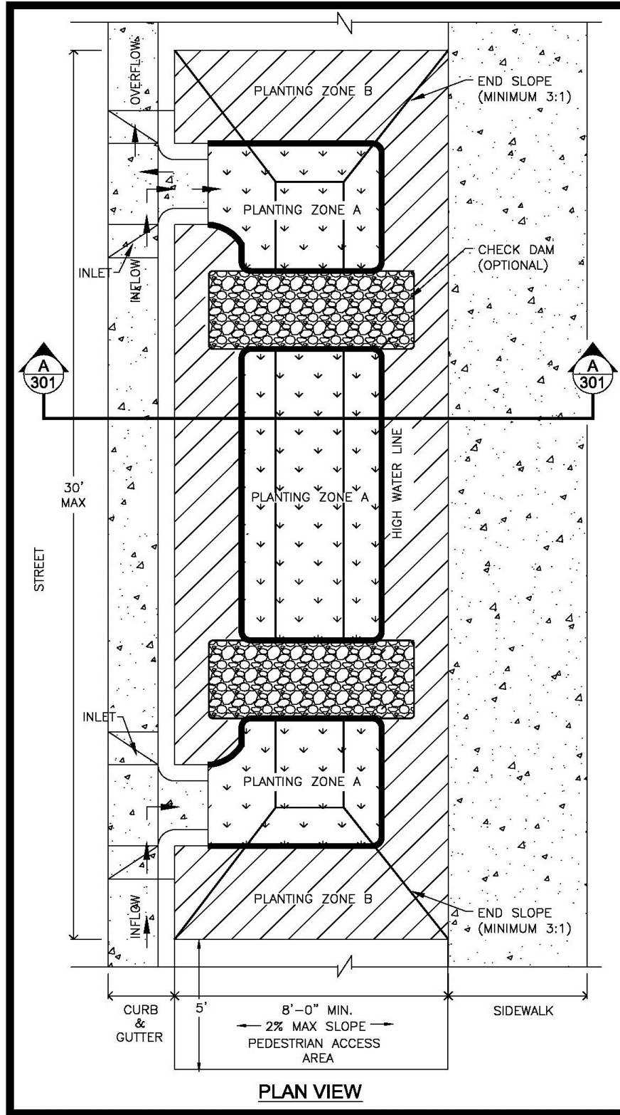
Figure GIP-02-05. Green Streets Swale Plan View (source: Portland, 2011)
