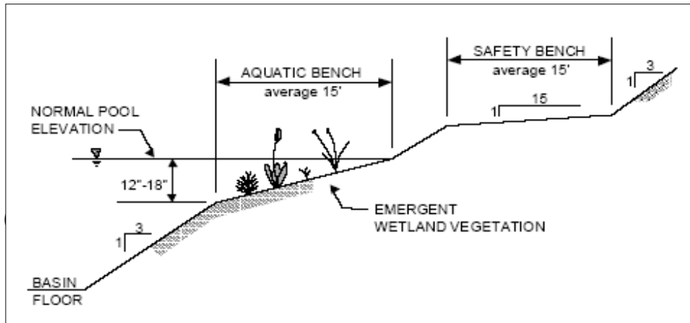
Figure TSS-01-05. Stormwater Pond Cross-Section with Benches
