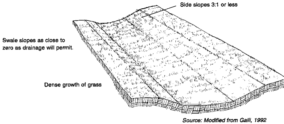
Figure TSS-07-01 Typical Grass Channel
