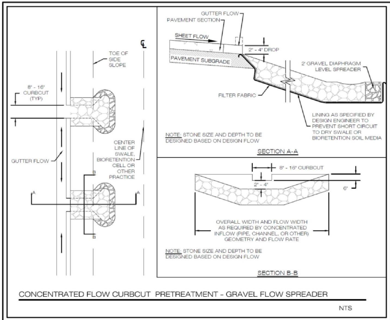
Figure GIP-01-06. Pre-Treatment Option – Gravel Flow Spreader for Concentrated Flow Outside of ROW (source: VADCR, 2010)
