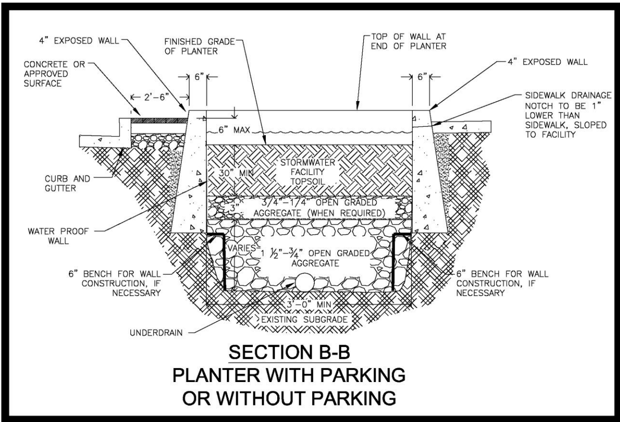
Figure GIP-02-08. Green Streets Planter Section View With or Without Parking (source: Portland, 2011)
