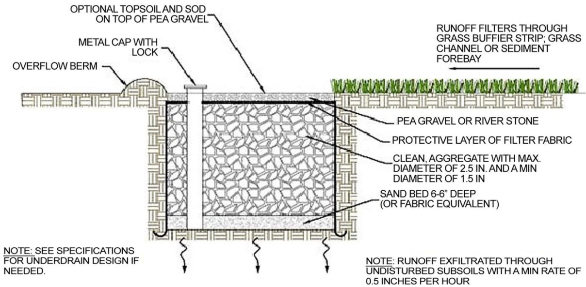
Figure GIP-04-01. Infiltration Plan and Section (VADCR, 2011)
