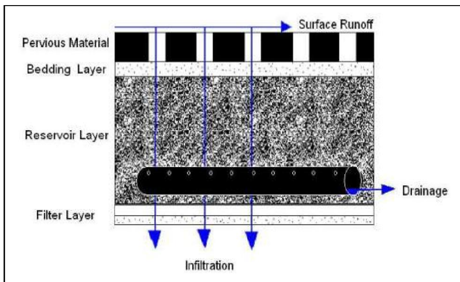
Figure GIP-03-01. Cross Section of Typical Permeable Pavement (Source: Hunt & Collins, 2008)
