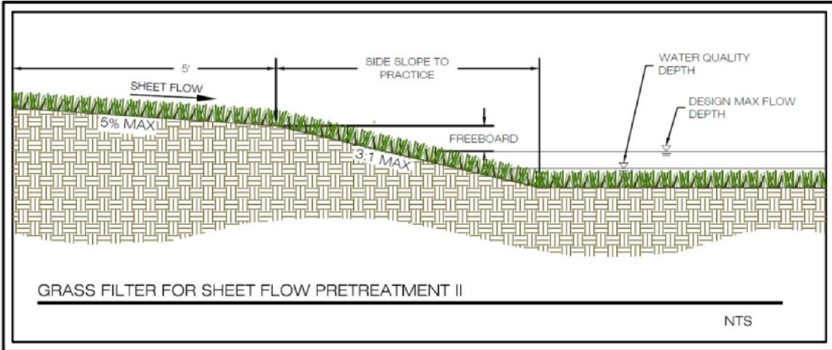
Figure GIP-05-05. Pretreatment I and II - Grass Filter for Sheet Flow (source: VADCR, 2011)
