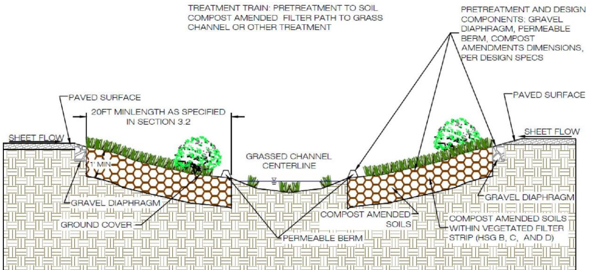
Figure GIP-07-04. Amended Filter Path to Downstream Grass Channel (or other treatment)(Source: VADCR, 2011)
