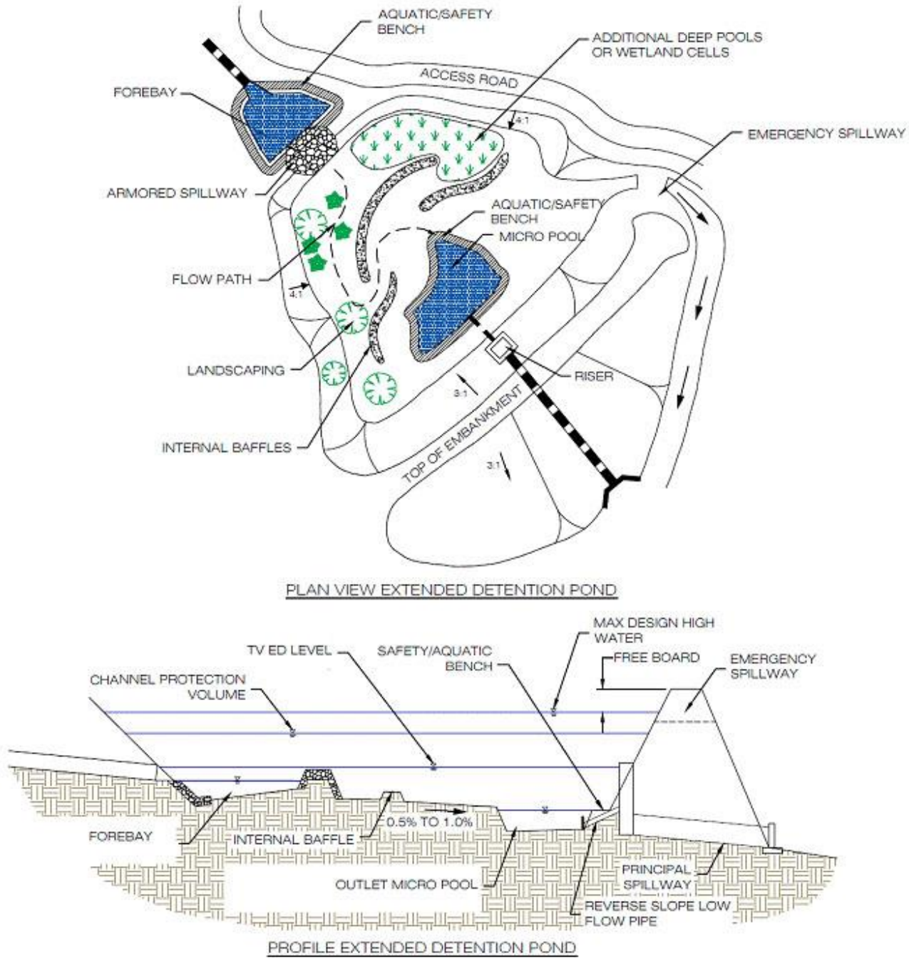
Figure GIP-06-01. Typical Extended Detention Pond Details (source: VADCR, 2011)
