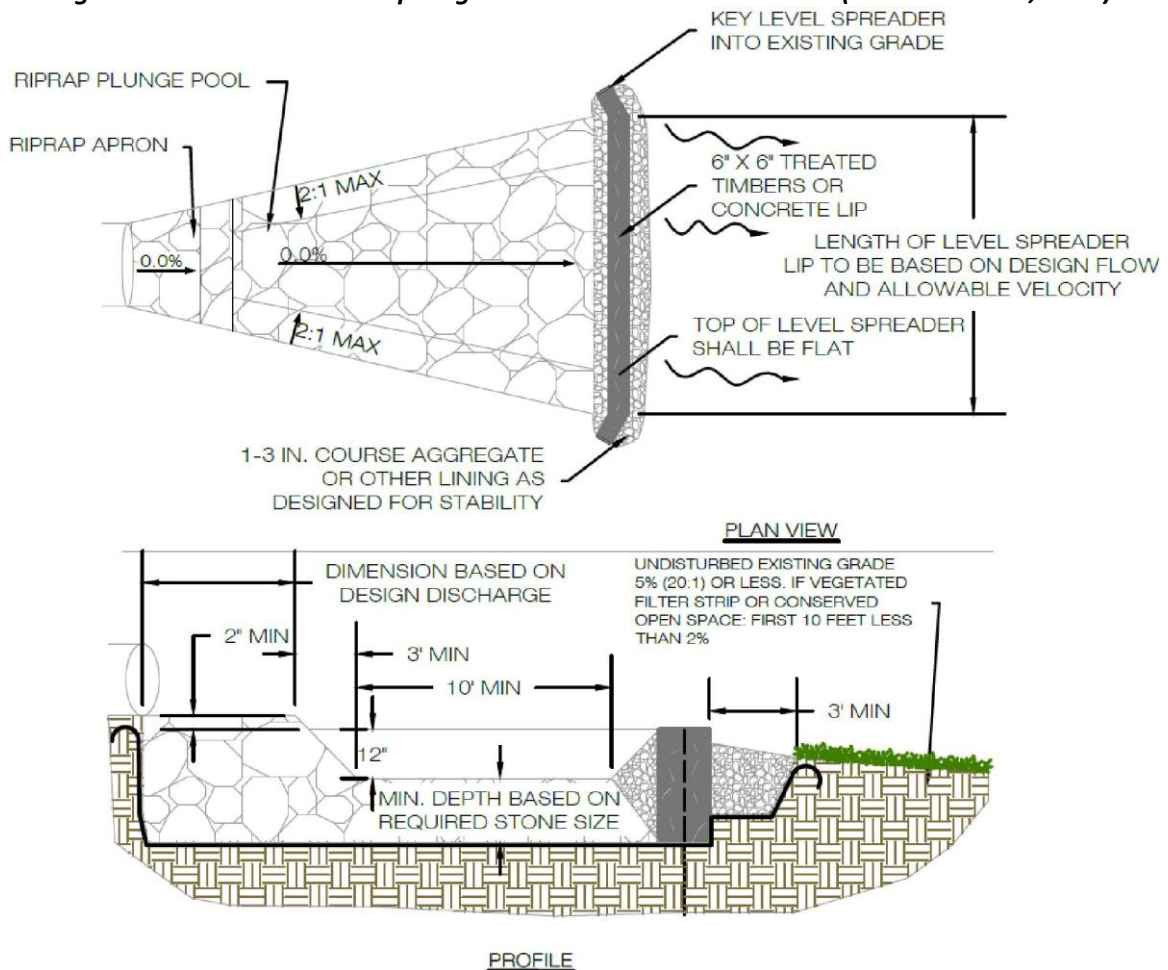
Figure GIP-09-07. Level Spreader: Pipe or Channel Flow to Filter Strip or Preserved Open Space (source: VADCR, 2011)
