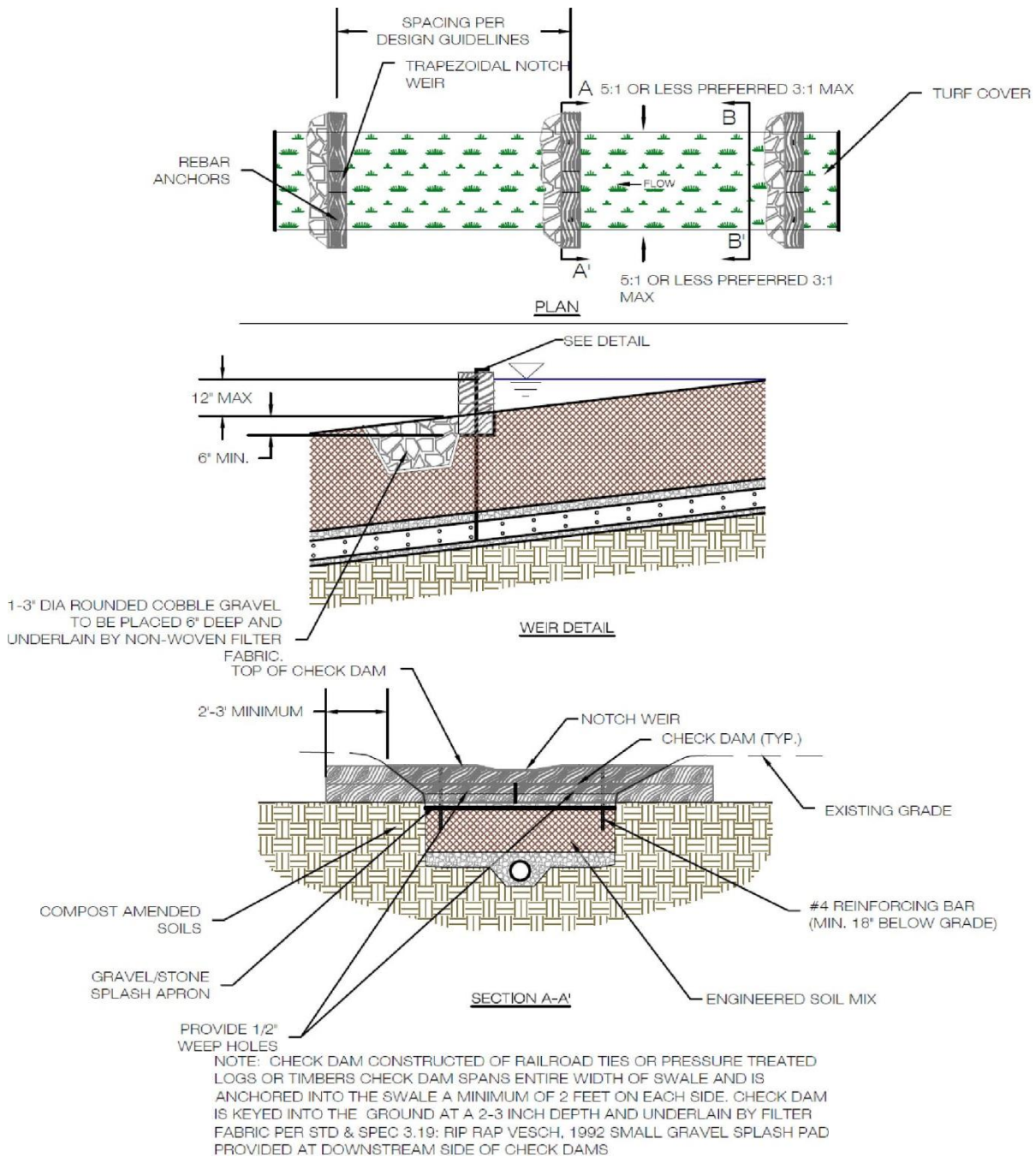
Figure GIP-05-04. Typical Detail for Water Quality Swale Check Dam (source: VADCR, 2011)
