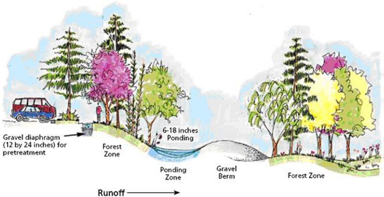
Figure GIP-09-01. Typical Sheet flow to Conserved Open Space (Hathaway and Hunt 2006)
