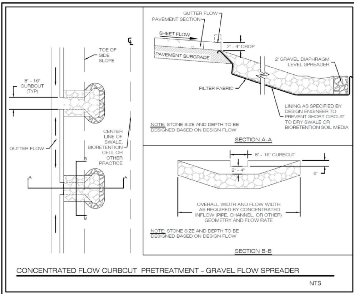
Figure GIP-05-07. Pre-Treatment – Gravel Flow Spreader for Concentrated Flow (source: VADCR, 2011)
