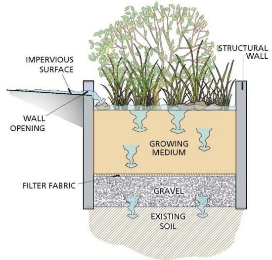
Figure GIP-02-07 Infiltration planter (Not for ROW). (Source: Portland Bureau of Environmental Services)
