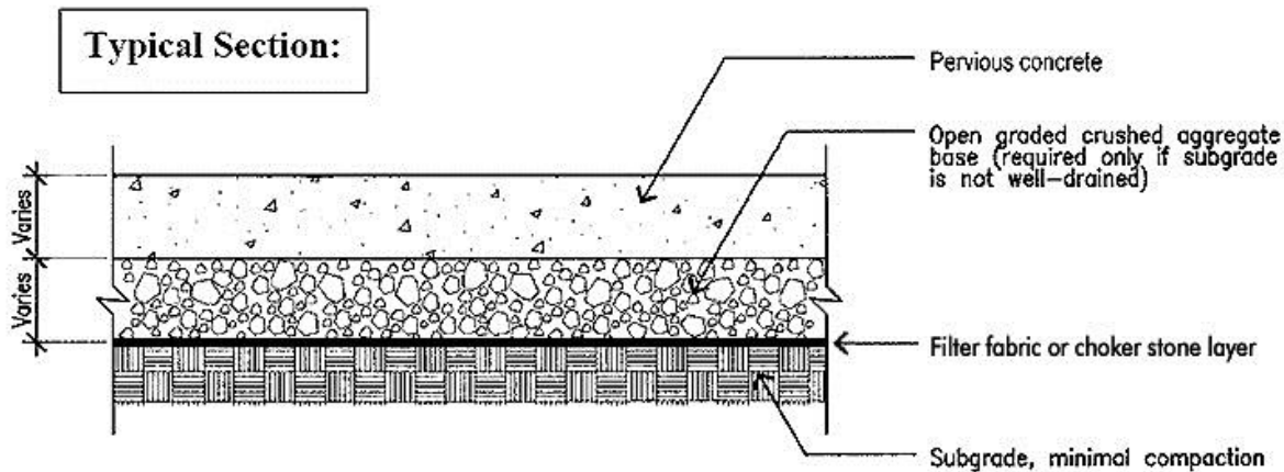
Figure GIP-03-03. Typical Detail of Pervious Concrete (Source: Portland, 2003)
