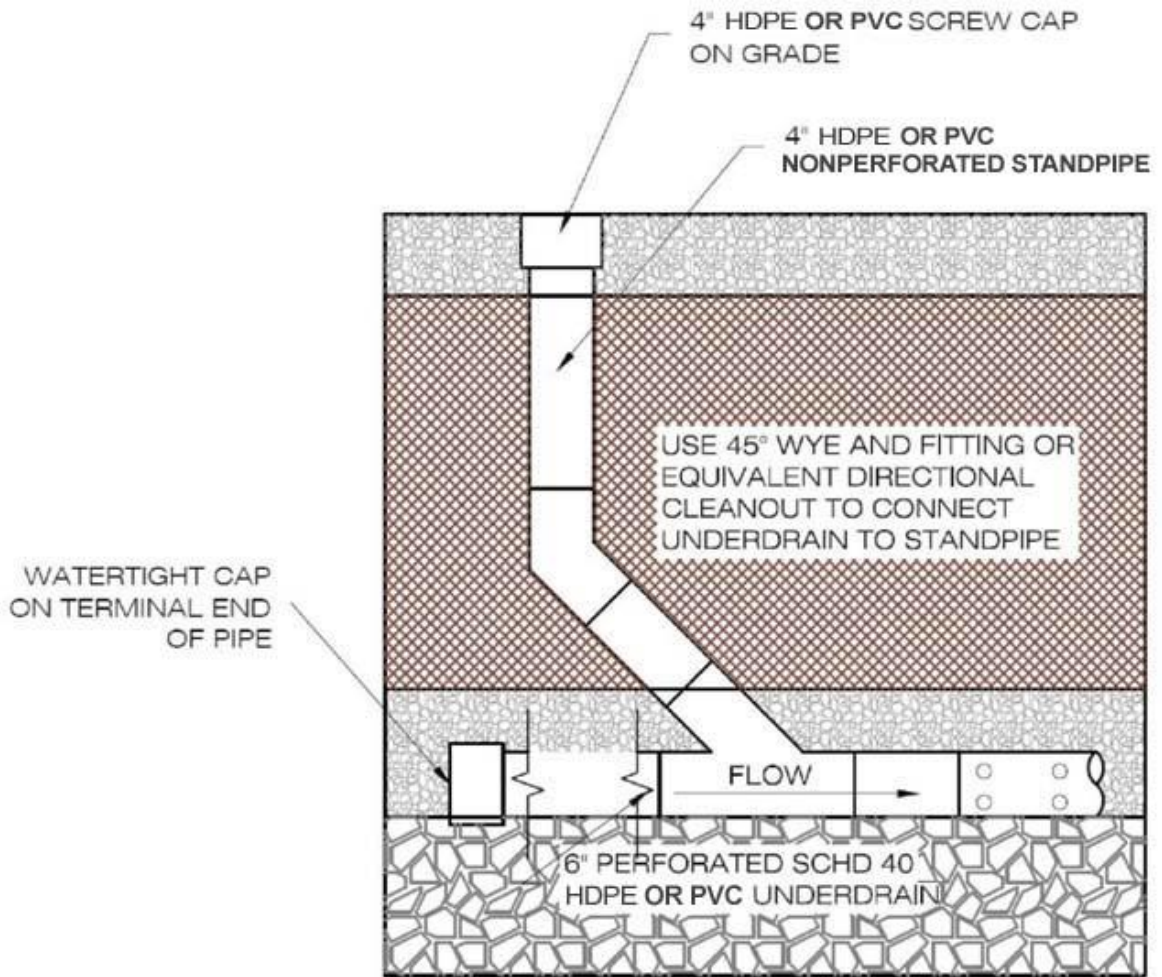
Figure GIP-01-B1. 1. 4" Cleanout Detail (source: VADCR, 2010)
